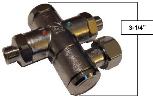
Mixing valve 3/8" compression inlets 1/2" NPT outlet
